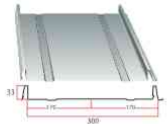
ลอนNova-Easy Snap
