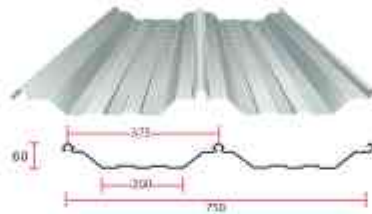
ลอนNova-Seam Lock
